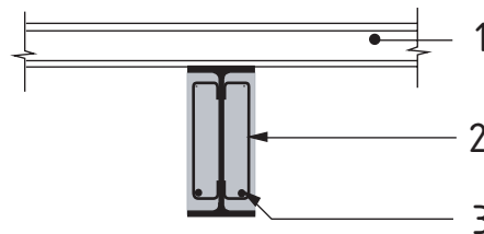
Figure 1.2: Composite beam comprising steel beam with no concrete encasement
